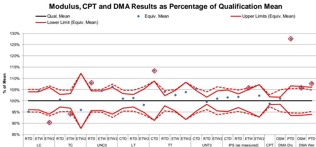
Figure 3-2 Summary of Modulus, CPT, and DMA means and Equivalence limits
